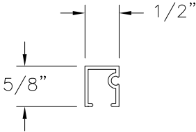
GLAZING BEAD(4806) ALUMINUM 6063-T5
