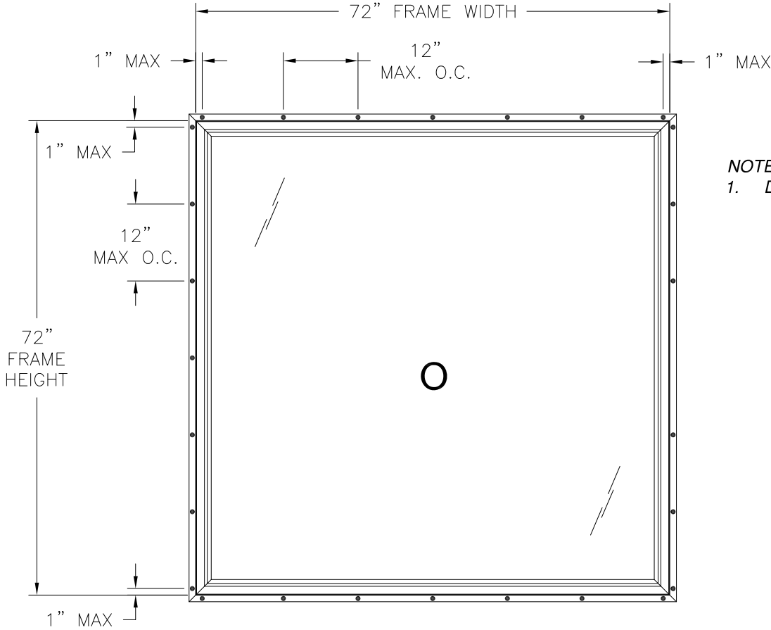
SERIES 101 PICTURE WINDOW EXTERIOR VIEW
